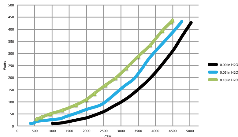
20" HLE AC Variable Speed Performance
